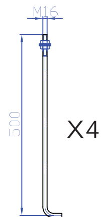
PERNO / ANCHOR BOLT 71-4539-48-48
